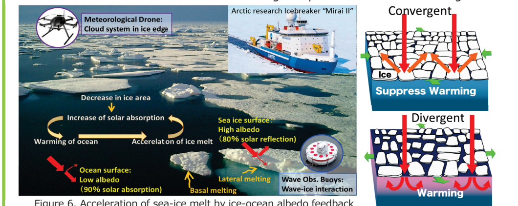
Figure 6. Acceleration of sea-ice melt by ice-ocean albedo feedback
