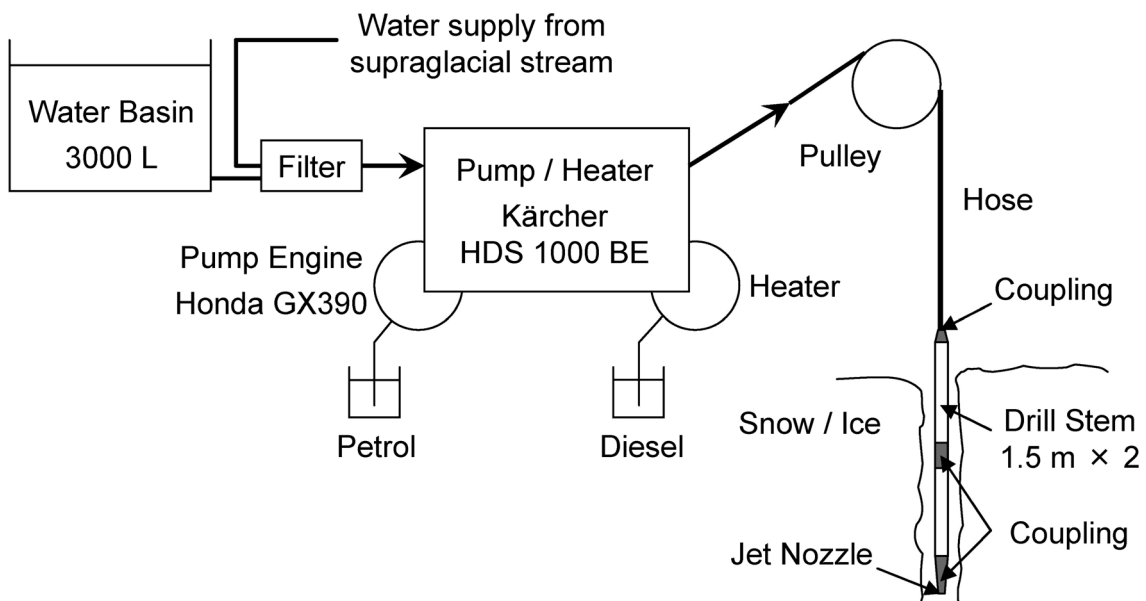
Fig. 2. Block diagram showing the configuration of the hot water drilling system constructed for this project.
