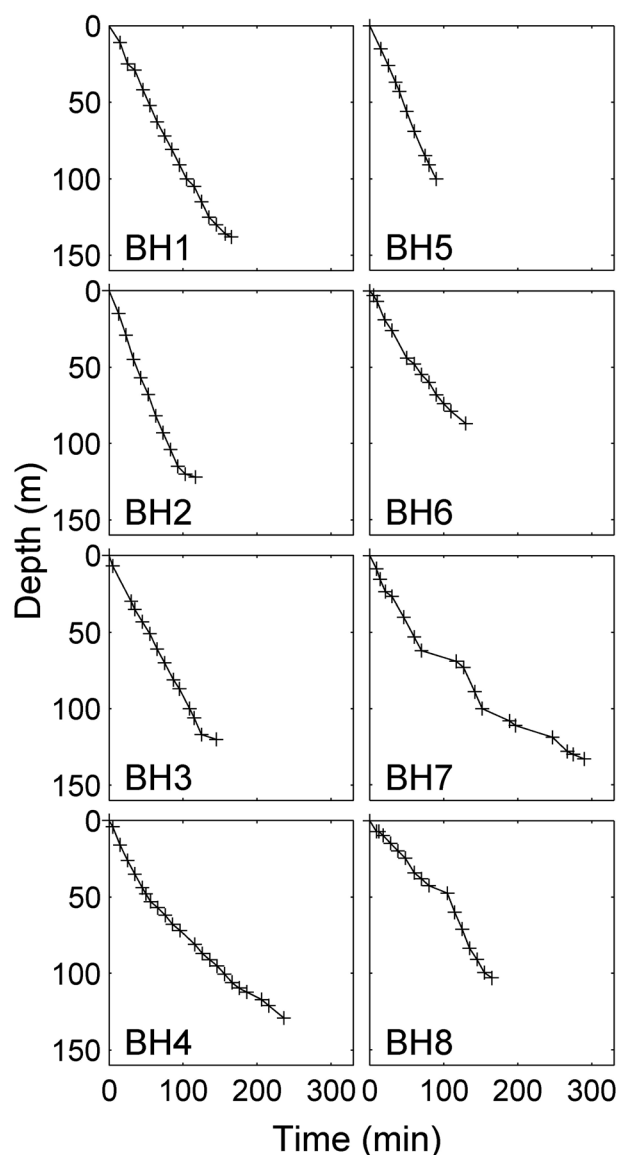
Fig. 8. Drilling depth as a function of drilling time for the boreholes from 2007.
