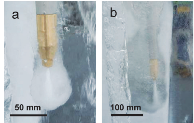
Fig. 5. Drilling nozzle and water jet in the ice block used for the test. The nozzle was lowered quickly in (a), while it was lowered slowly to enlarge the borehole diameter in (b).
