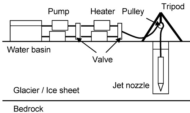
Fig. 1. Schematic of a hot water drilling system.
