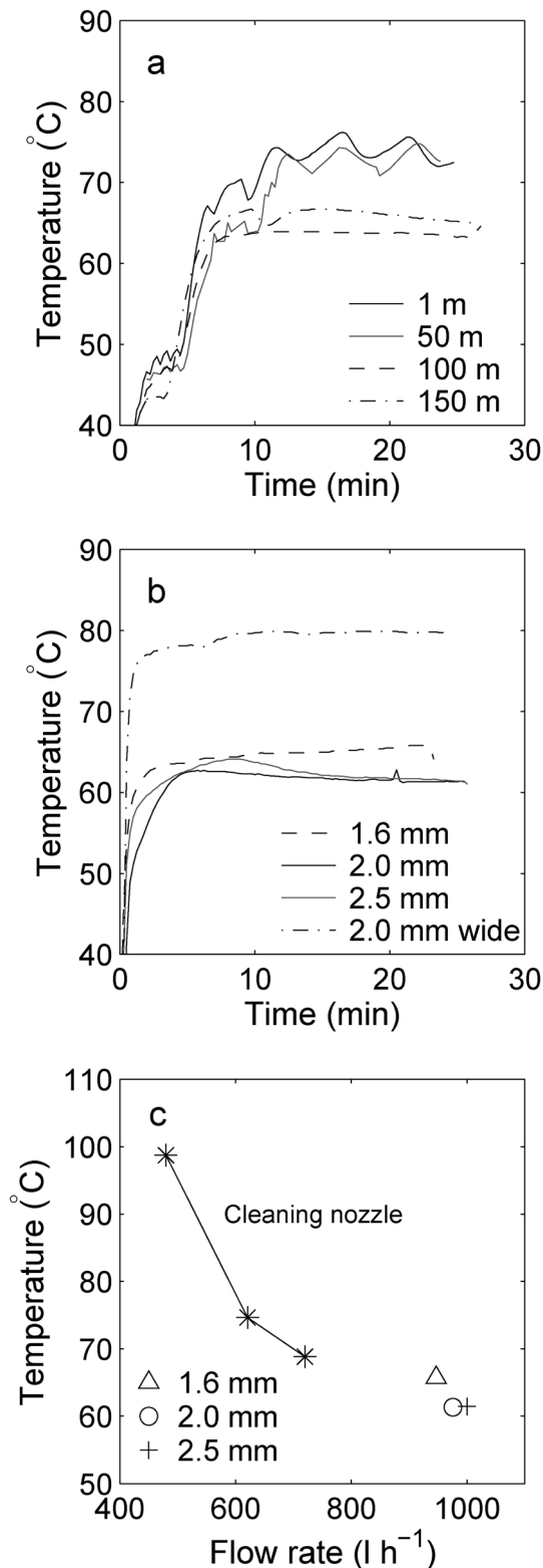
Fig. 4. Water jet temperature vs. time with (a) various hose lengths and (b) various jet nozzle diameters. (c) Flow rates and water jet temperatures obtained with the three jet nozzles and the cleaning nozzle.
