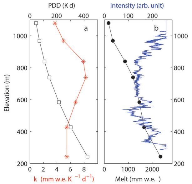
Fig. 6. (a) PDD (□), degree-day factors (*) and (b) total melt amount at Q1201–Q1207 computed for the entire summer melt season in 2012. Blue line in (b) is the brightness intensity of the ALOS PRISM image (25 August 2009; see Fig. 1) along the survey route.
