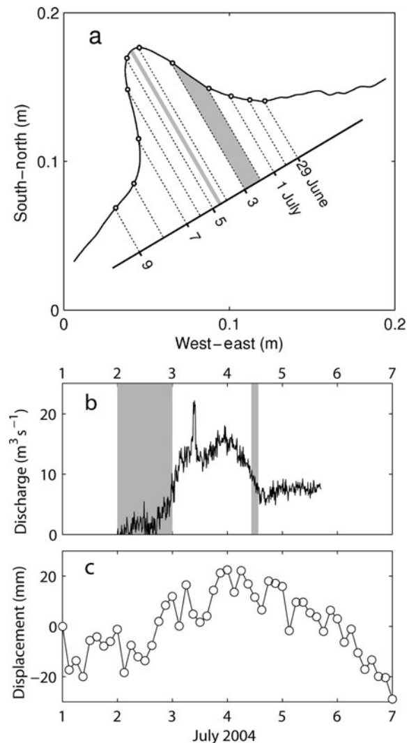
Fig. 7. (a) Plan view of the stake motion at GPS42. The open circles on the smoothed trajectory indicate the locations of the stake at 0000 h. (b) Water discharge from the lake. The shaded bands show the day of the maximum northwest displacement and the timing of the reversal of the transverse ice motion. (c) Vertical displacement at GPS42 relative to the elevation at 0000 h on 1 July.
