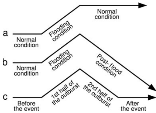
Fig. 6. Schematic diagrams showing the trajectories of stake motion during the lake outburst.
