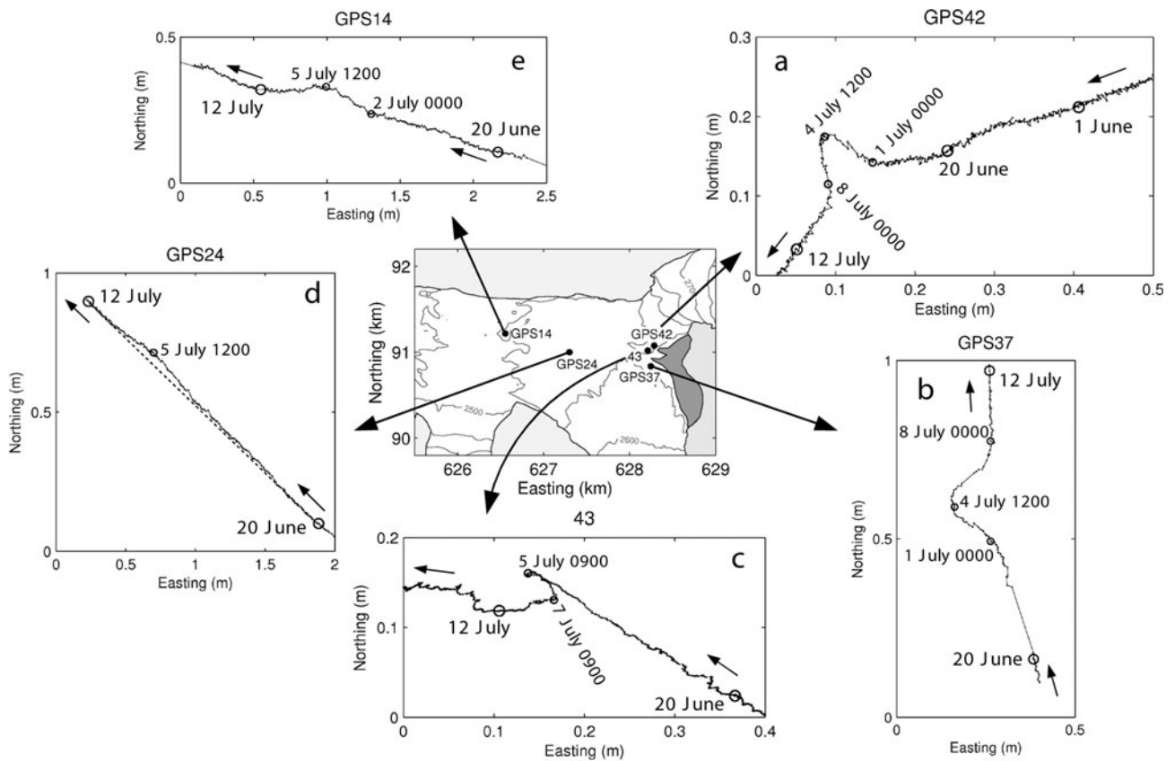
Fig. 5. Plan view of the stake motion at each survey site. The contour lines on the map indicate the surface elevation at intervals of 50 m. The vertical axes in (d) and (e) are exaggerated by a factor of two to emphasize the transverse stake motion. The dotted line in (d) connects the stake positions at 0000 h on 20 June and 12 July.
