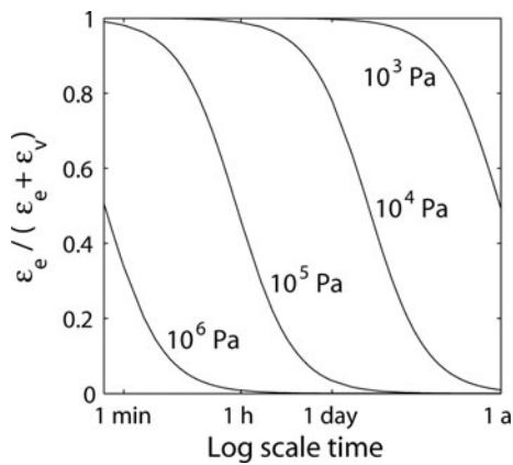
Fig. 8. Ratio of elastic to total strain under various stresses ( \tau ), as calculated by Equation (1).
