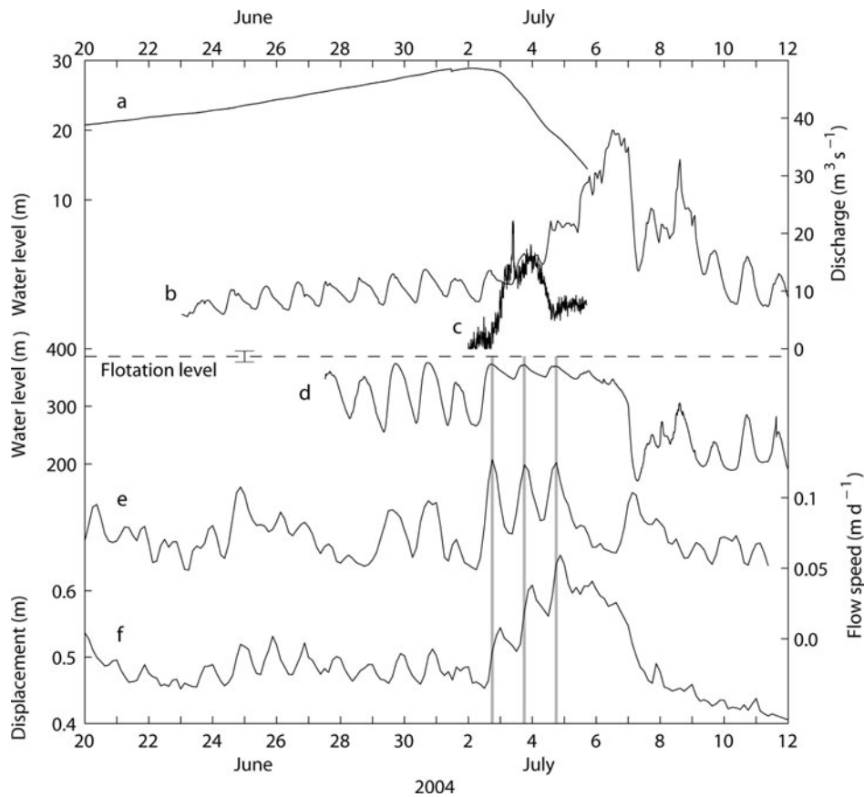
Fig. 3. Time series of (a) lake water level, (b) discharge from the glacier, (c) discharge from the lake, (d) water level in borehole BH430 and (e) horizontal flow speed and (f) vertical displacement at GPS14. The vertical displacement is relative to the elevation at the beginning of the GPS survey on 15 April. The dashed line indicates the flotation water level at the borehole site with an error bar. The vertical gray lines show the correlation of the water level, flow speed and vertical displacement.
