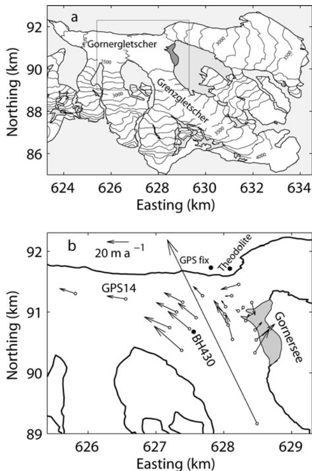
Fig. 1. (a) Map of Gornergletscher and Grenzgletscher with surface contour lines at intervals of 100 m. The study area is indicated by the box. (b) Location of the GPS and theodolite survey stakes with annual flow vectors obtained for the period October 2003 to September 2004. The borehole drilling site is labeled BH430.
